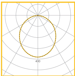
Prismatic Diffuser 56W LED LOR = 100.0% SHR MAX = 1.55
