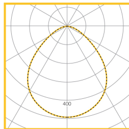
Hexaprism Optic 41W LED LOR = 100.0% SHR MAX = 1.58
