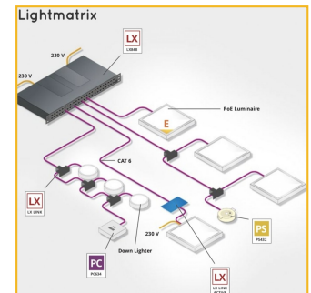
Power over Ethernet Topology
