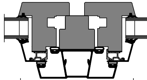
Mullion DK015
