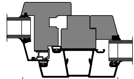
Mullion DK017
