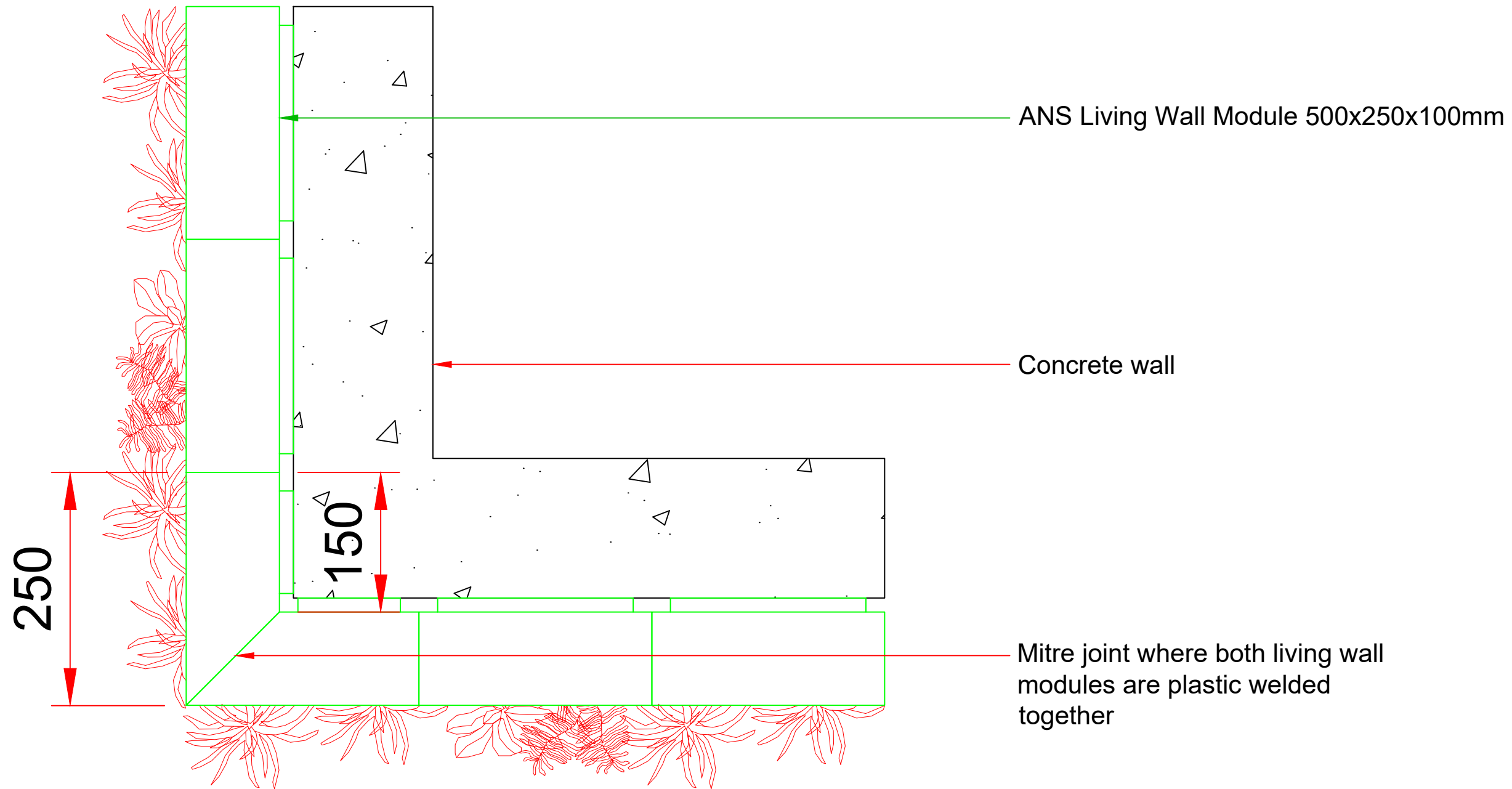
Plan View Scale: 1:5
