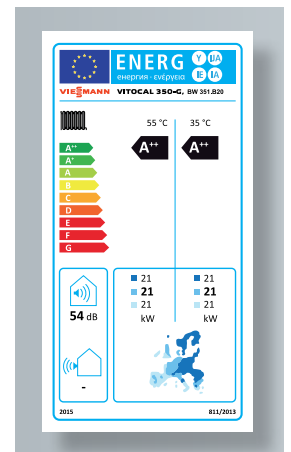
Energy efficiency label Vitocal 350-G, BW 351.B20
