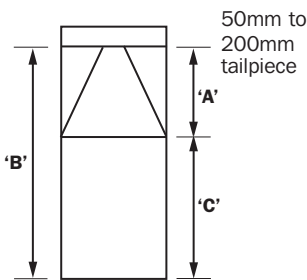
Glass Below Calculation
