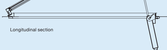
Ventria-O, uninsulated open
