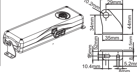
swivel bracket
