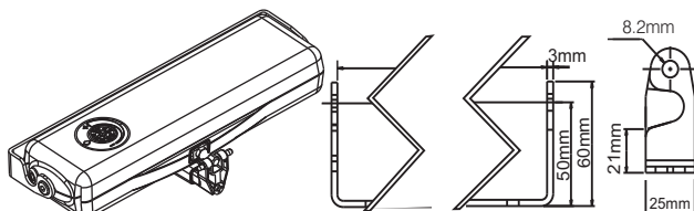
long bar swivel bracket
