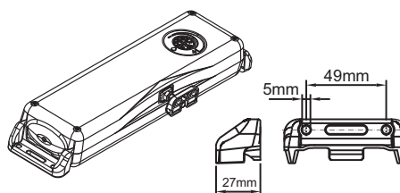
swivel bracket
