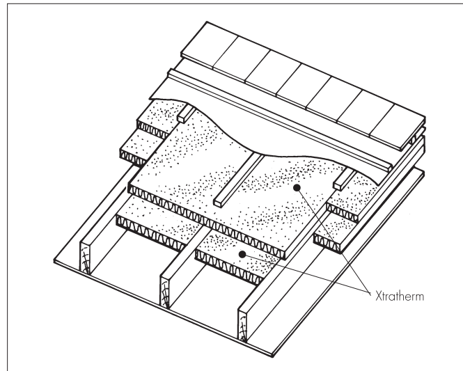
Figure 1 Typical installation
