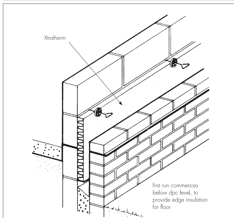
Figure 1 First run of boards
