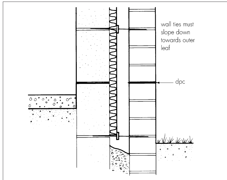
Figure 2 Detail of wall ties
