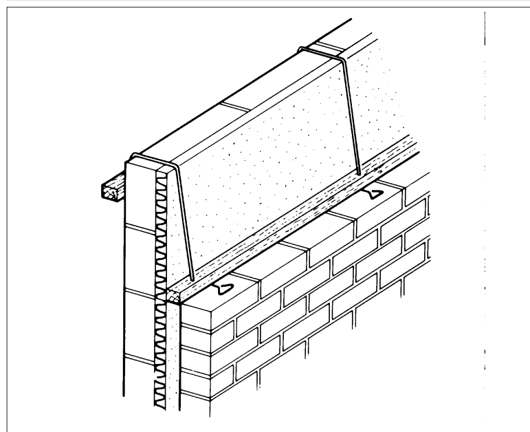
Figure 3 Use of cavity batten
