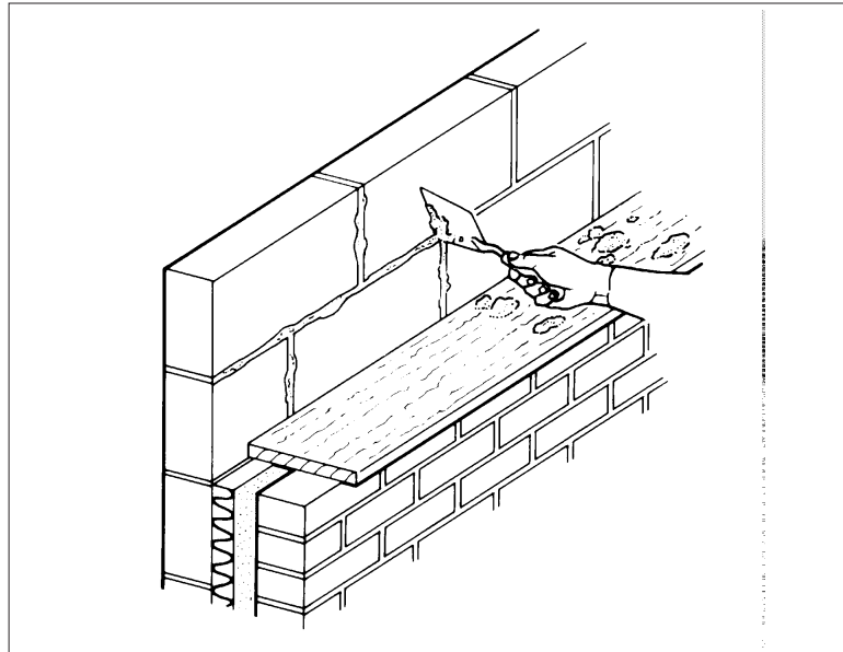
Figure 4 Use of cavity board
