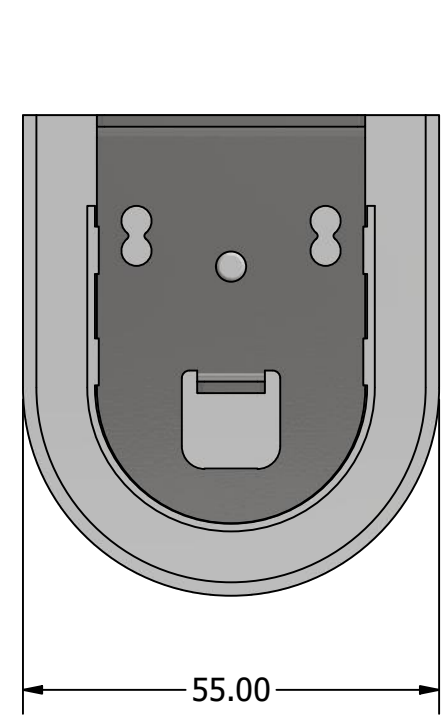
Sirios standard bracket Excluding bracket cover
