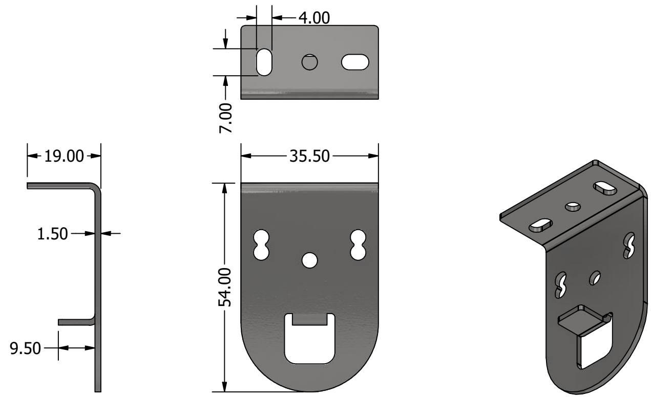
Sirios standard bracket Excluding bracket cover
