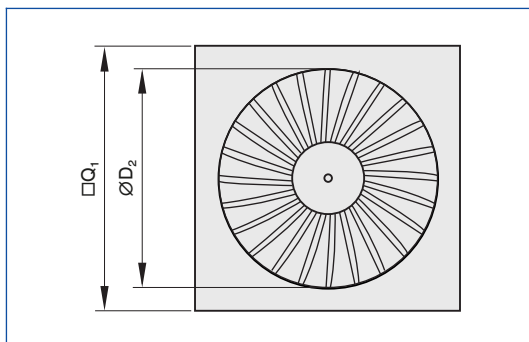
Diffuser face TDF-SA-Q
