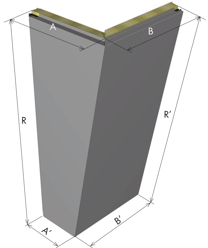
Fig. 2.8: Corner under an angle
