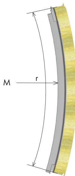
Fig. 1.12b: Curved elements - Concave
