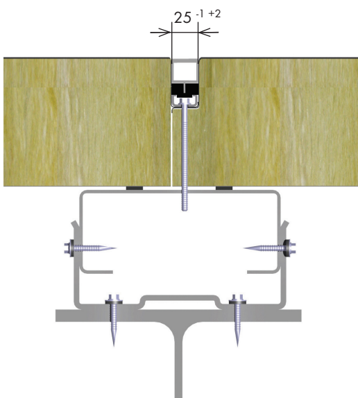
Fig. 1.6: TRANSVERSAL and LONGITUDINAL joint for both horizontal installation methods
