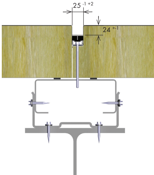
Fig. 1.2: Facade element QO B - Horizontal installation
