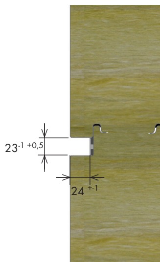
Fig. 1.6: TRANSVERSAL and LONGITUDINAL joint for both horizontal installation methods
