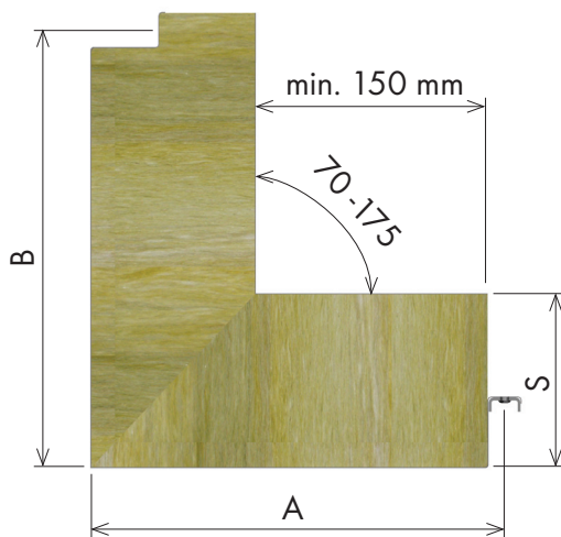
Fig. 2.1: L corner shape
