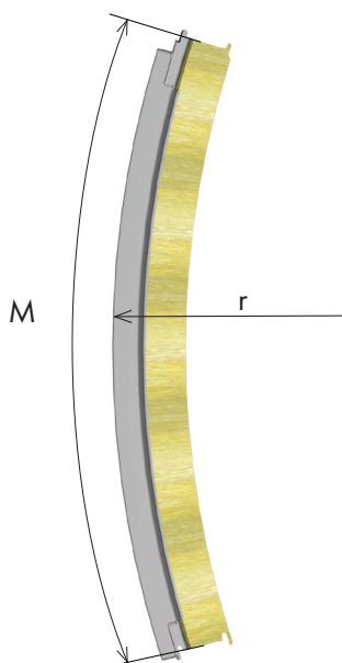
Fig. 1.12a: Curved elements - Convex
