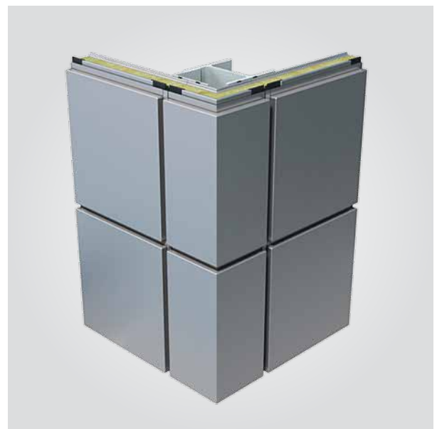
| Corner detail
