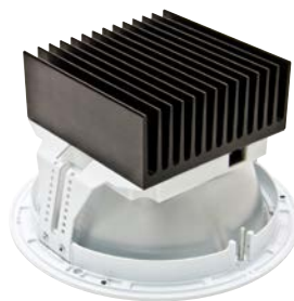
Body and heat sink
