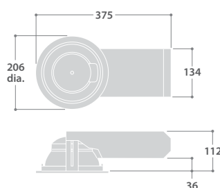
Cut-out - 180 dia. Minimum void depth - 140
