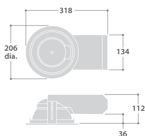
Cut-out - 180 dia. Minimum void depth - 105
