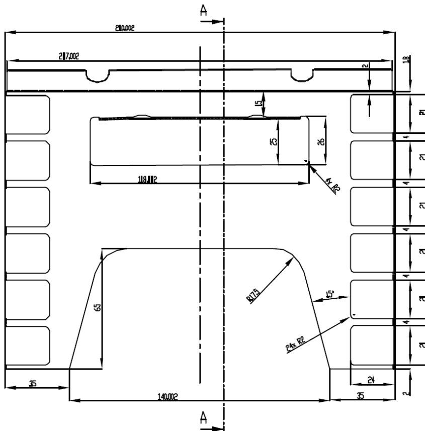
Figure A.1.1 The ICF wall construction design as provided by MCG Group Ltd (note: there are three modifications. (A) An external render of 12.5mm has been included. (B) A 50mm cavity with 50x50mm timber studs at 400mm centres has been included. (C) An internal plasterboard finish of 12.5mm has been included.
