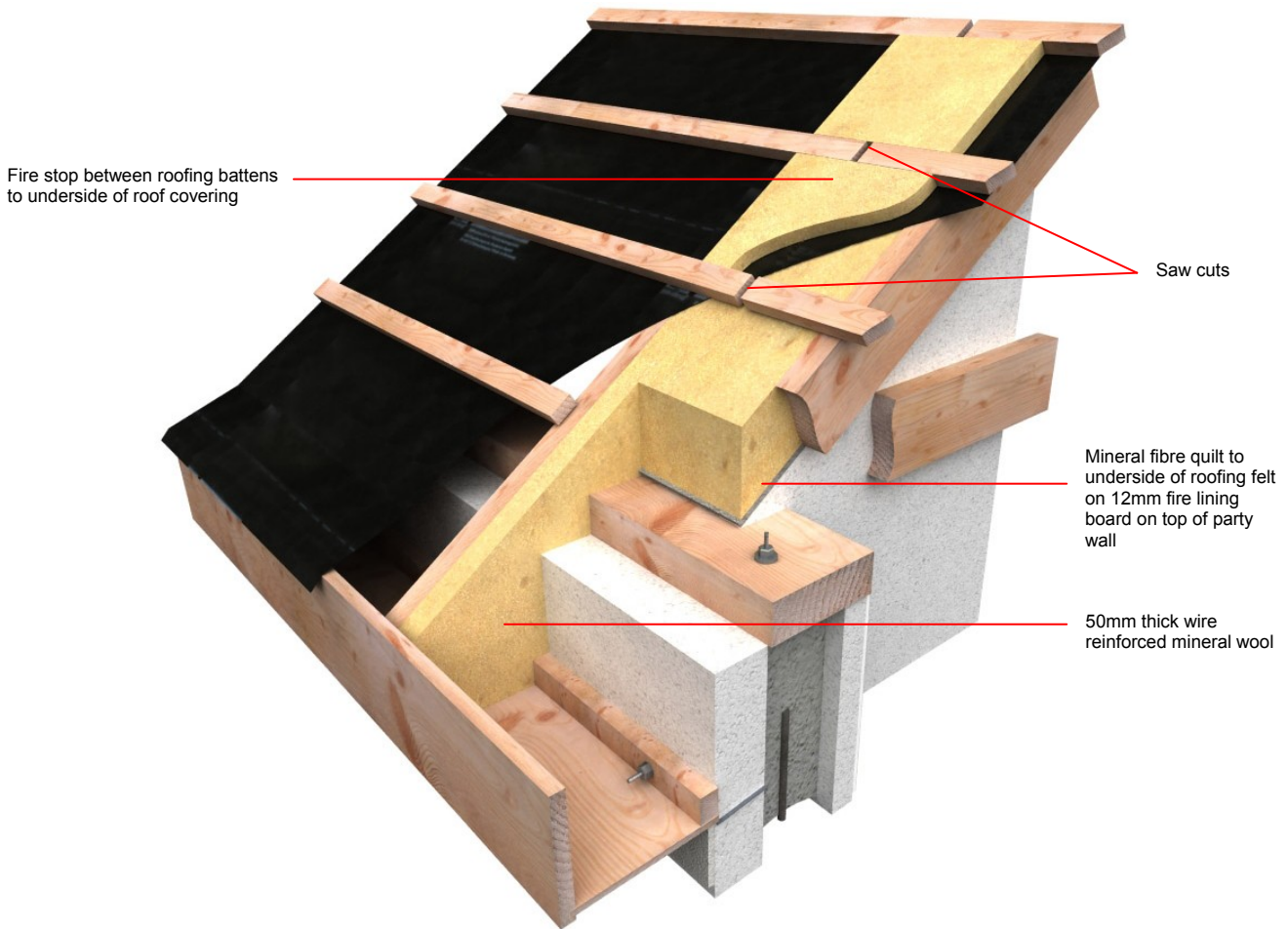
Figure 15: Fire Stopping at Party Wall
