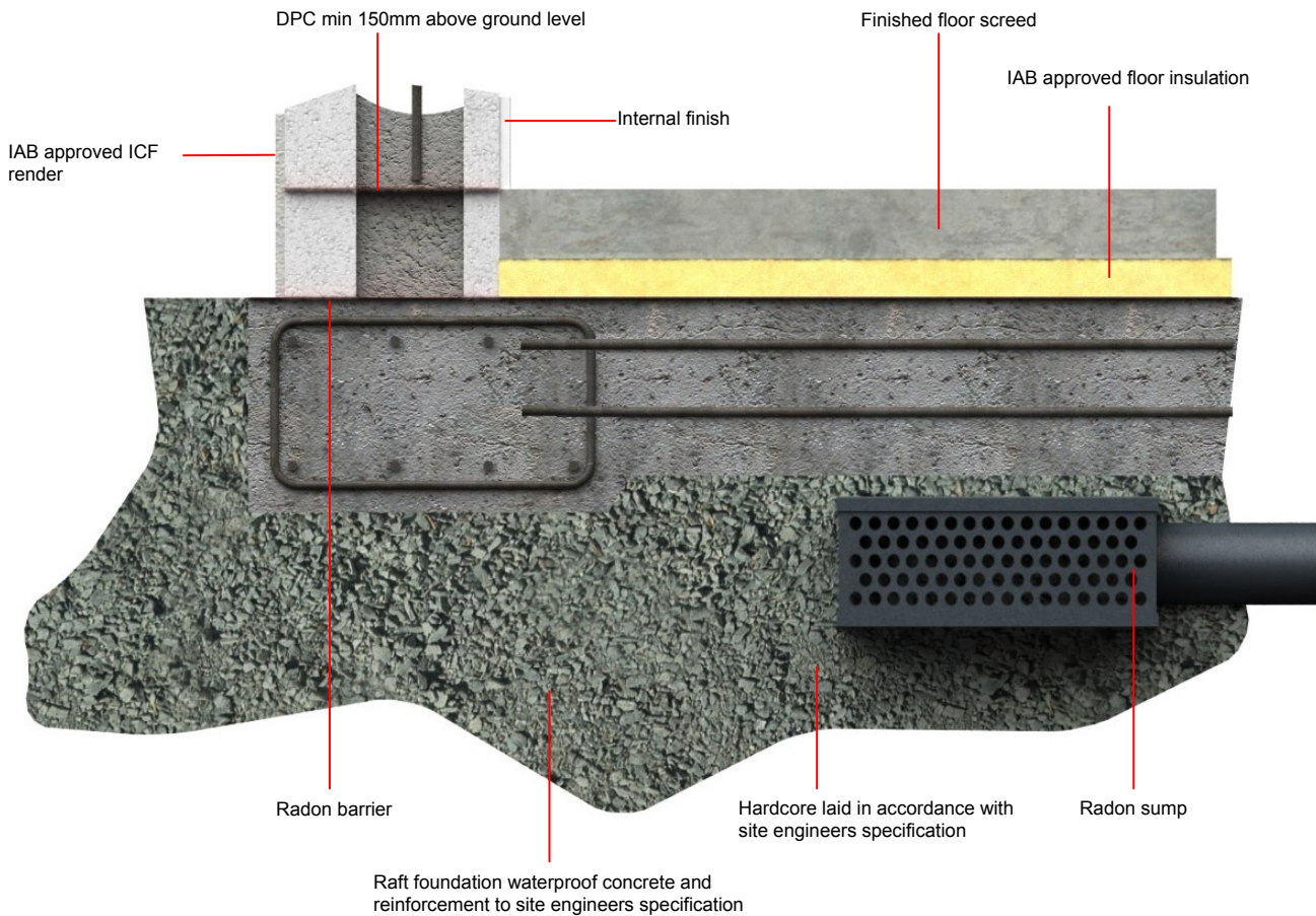
Figure 2: Raft Foundation Details
