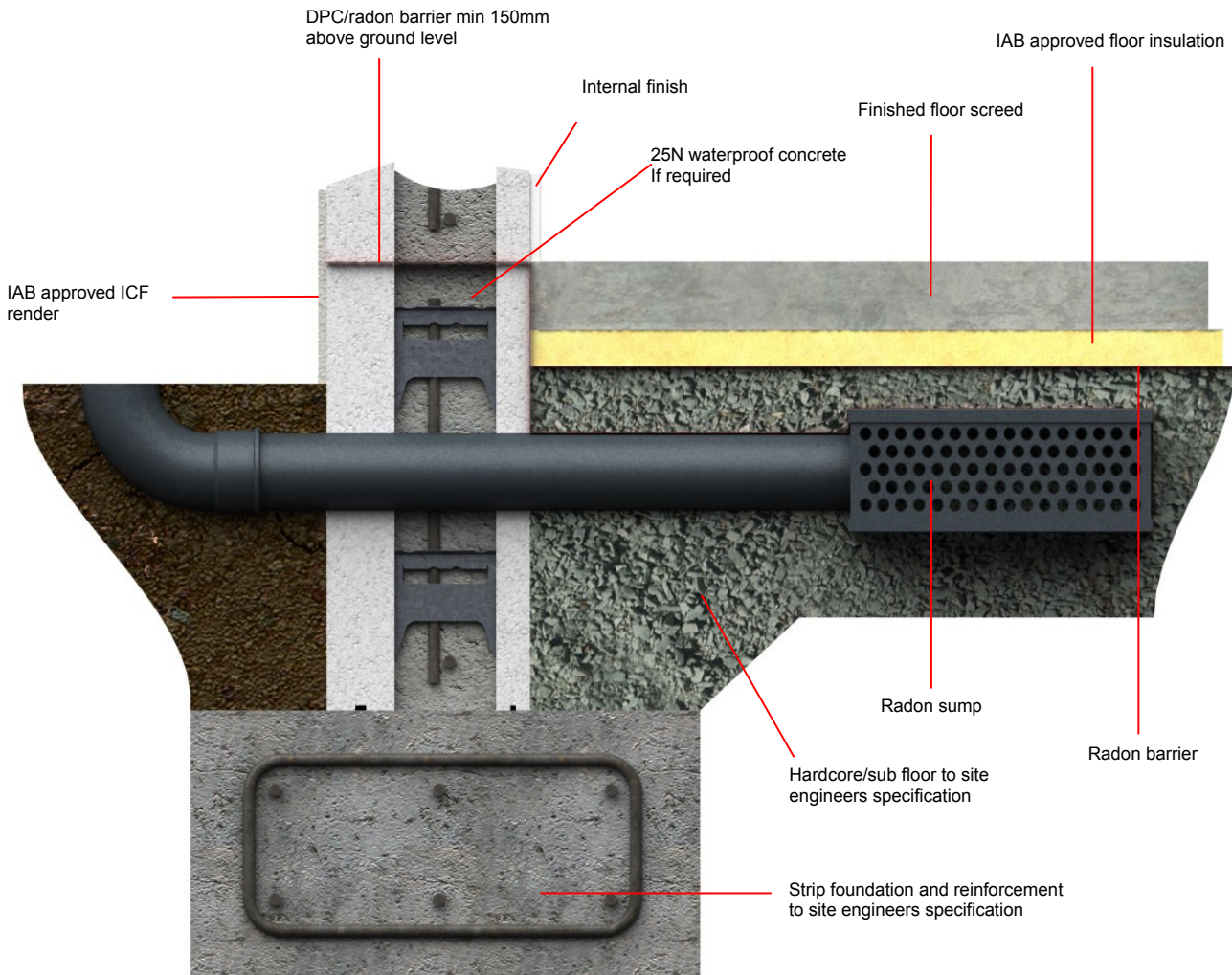
Figure 1: Strip Foundation Details
