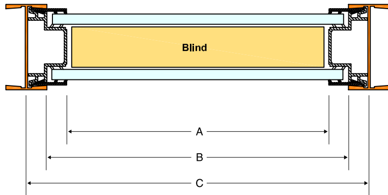
flexplus - glazing setting out details
