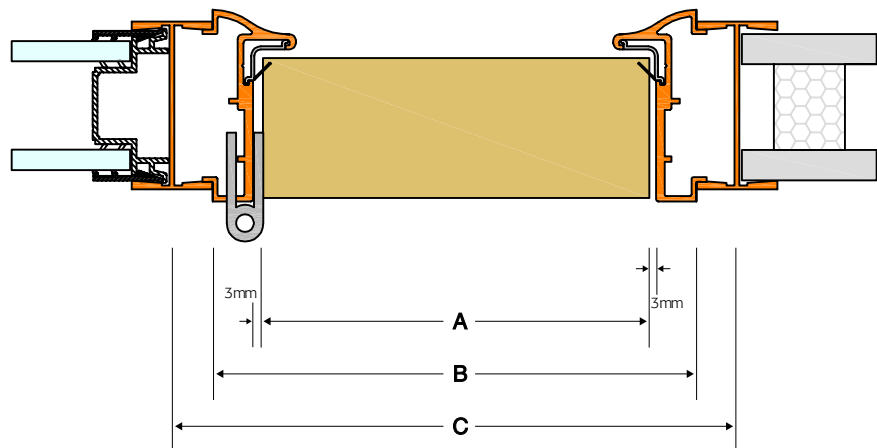
flexplus - door frame setting out details
