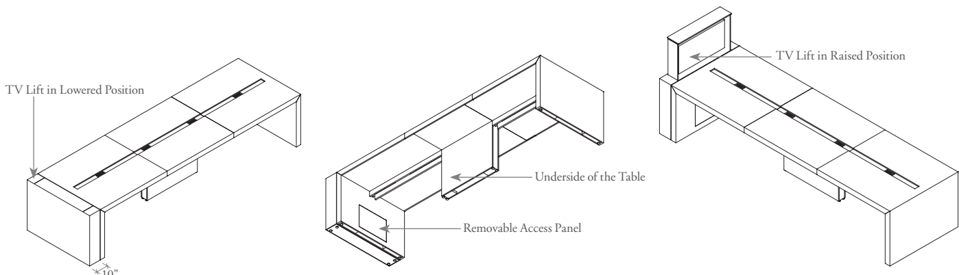
Installed at one end of the table and will add 10" to the overall table width.
