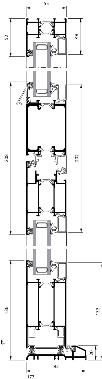
Coupe verticale 1B-B' Vertical cross section Corte vertical
