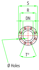
Flange UNI-PN6
