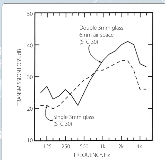
Figure 3. The effect of a small airspace on TL of double glazing
