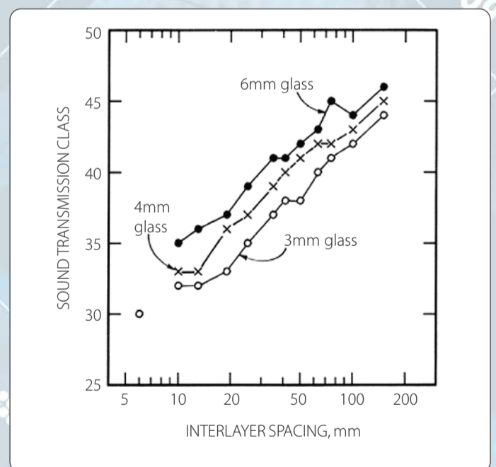
Figure 2. Sound transmission class (STC) versus interpane spacing for double glazing
