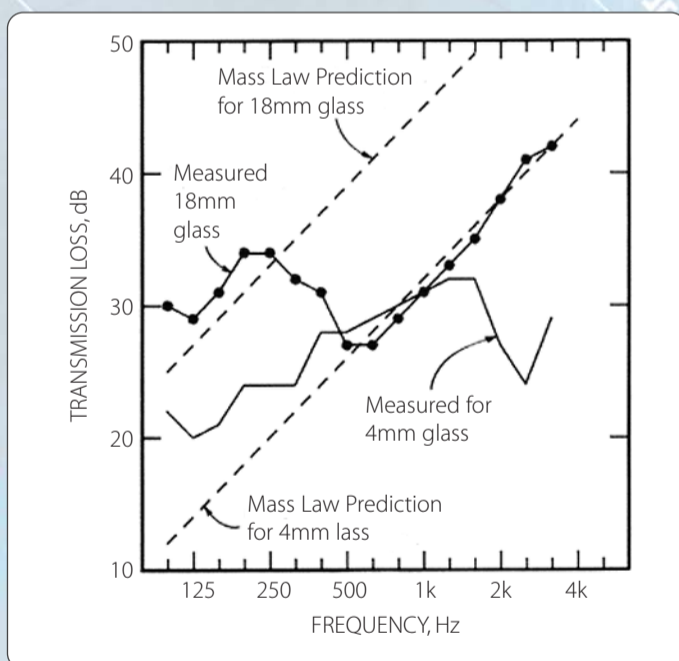
Figure 1. Sound transmission loss (TL) for sealed single glazing
