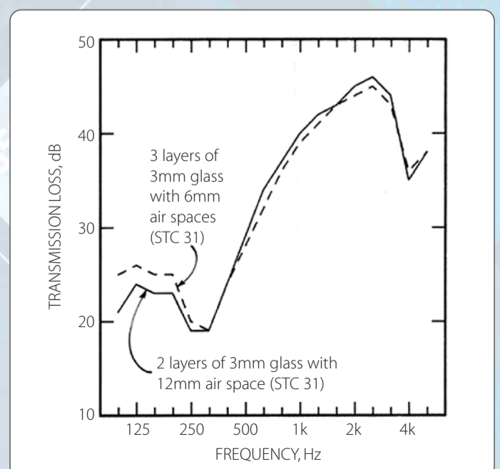
Figure 4. TL of double and triple glazed windows
