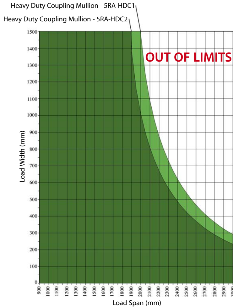
Size Limits for H/Duty Coupling Mullions at 1200Pa wind load (100MPH wind speed)
