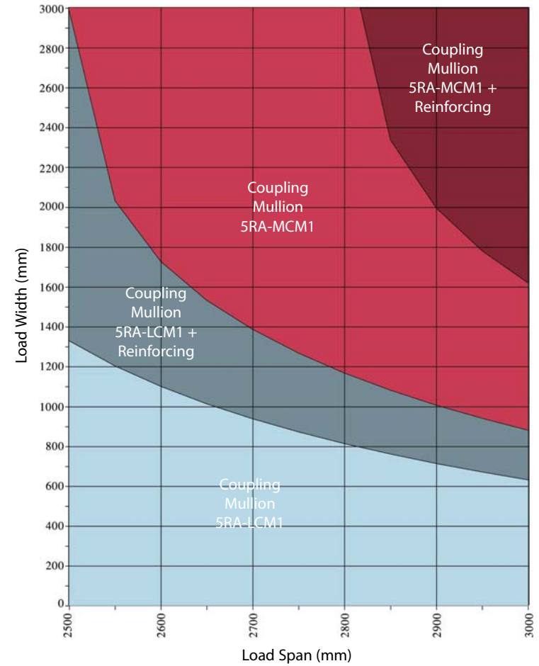
Size Limits for Coupling Mullions at 2000Pa wind load (130MPH wind speed)
