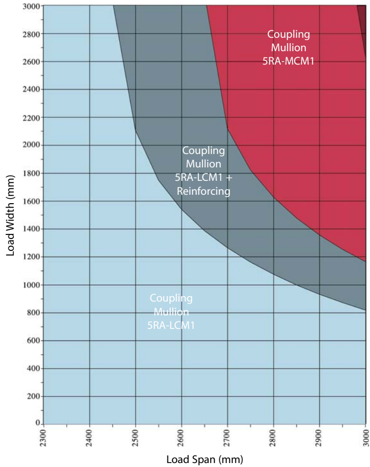
Size Limits for Coupling Mullions at 1600Pa wind load (115MPH wind speed)
