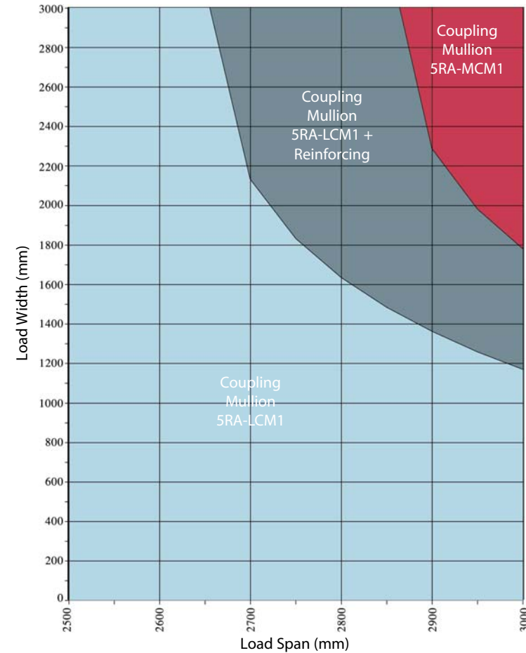
Size Limits for Coupling Mullions at 1200Pa wind load (100MPH wind speed)
