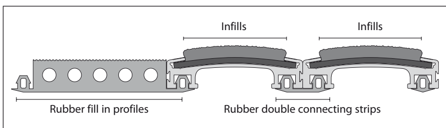
Nuway grid with rubber insert
