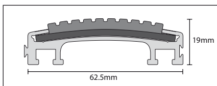
Nuway grid with rubber insert
