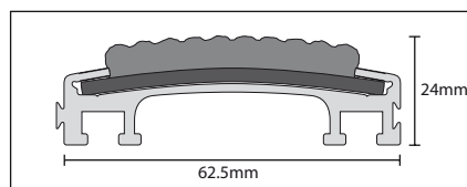
Nuway grid with burford insert
