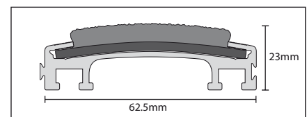
Nuway grid with Coral insert
