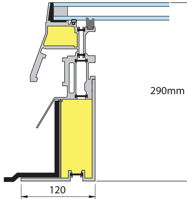
Standard Glazed Rooflight
