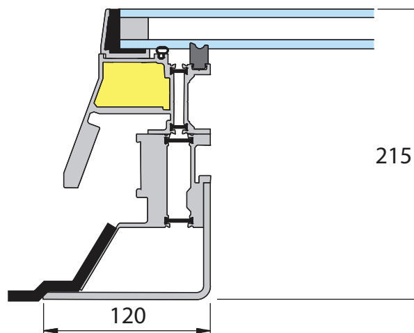
Reduced Upstand Glazed Rooflight
