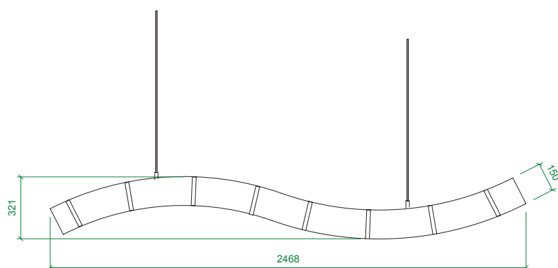
Wave design ELEVATION VIEW
