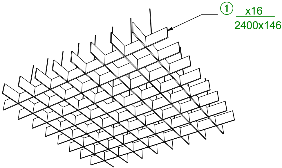
Grid baffles ISO VIEW
