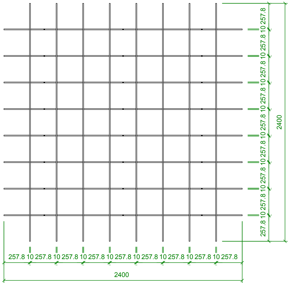
Grid baffles PLAN VIEW
