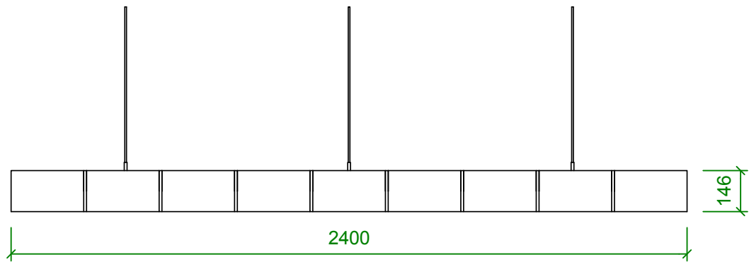
Grid baffles ELEVATION VIEW
