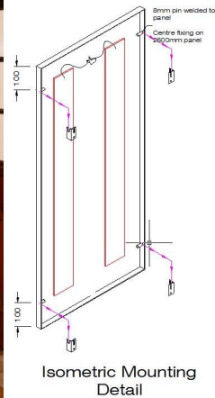
Right: Solray Radiant Panels either side of the gallery doorway Left: Isometric Mounting Detail taken from the Working Drawing
