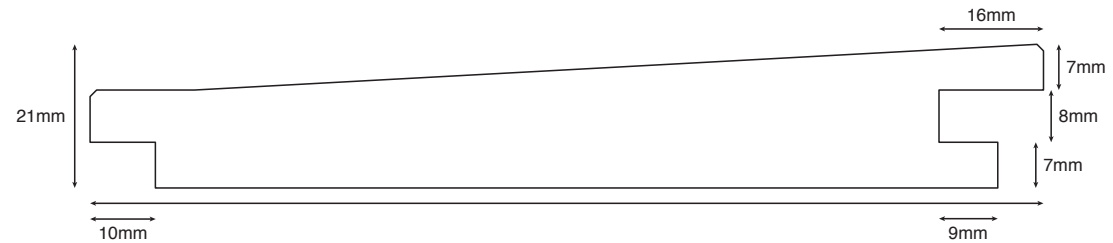
SAWFALLING I-IV 22 X 146MM REBATED BEVEL
