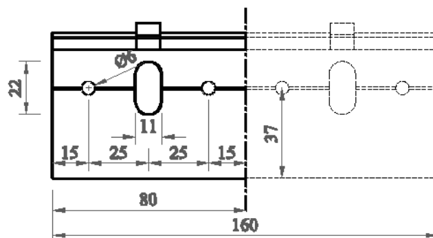
Type N62 - Single
