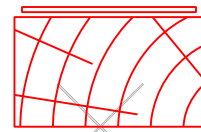
Batten-staff bead Standard softwood ground. For cill & right jamb. Mirror for head & left jamb.
