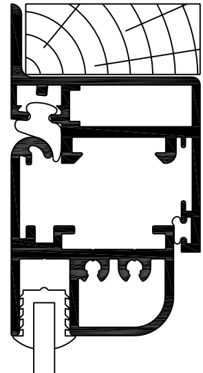
SINGLE CASEMENT
