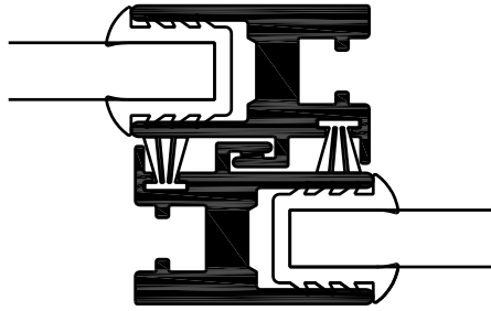
SECTION E-E
