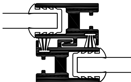
SECTION E-E
