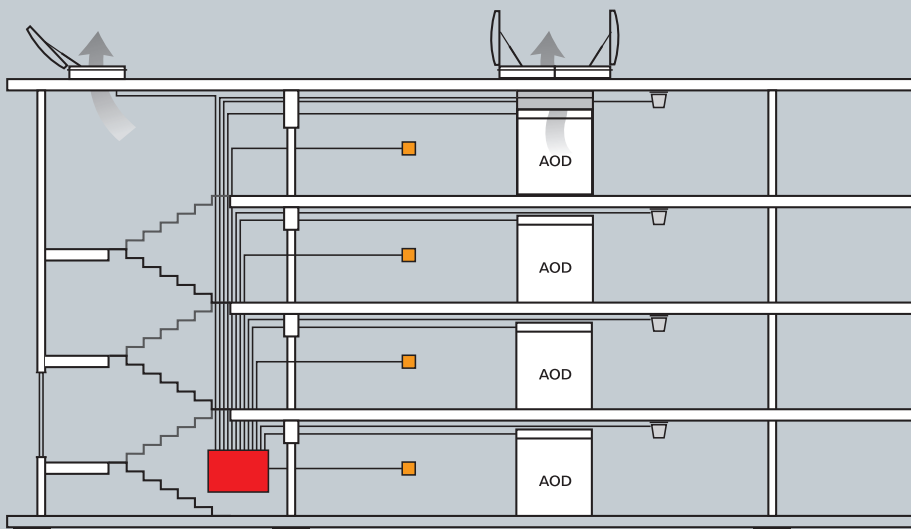
230v required for Central Control Point
