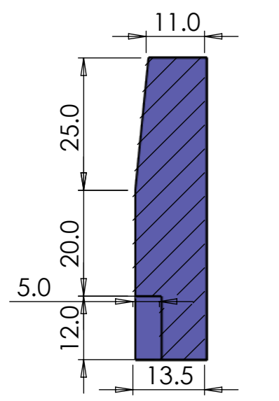
SECTION B-B SCALE 1:1
