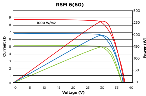
Characteristic Curves: Isc, Voc vs Radiation Intensity
