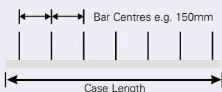
STARTABOX Fixing in Formwork
