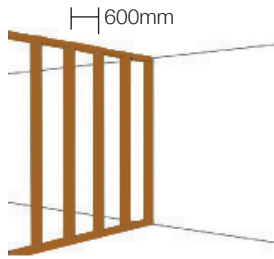
1. Vertical studs at 600mm centres.
