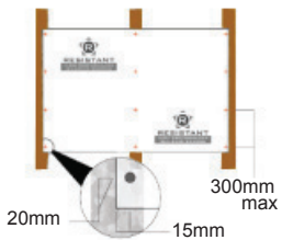
3. 12mm Multi-pro MoistSure for walls. Space fixings minimum 20mm from bottom & 15mm from side at 300mm intervals. Ensure screws are countersunk.
