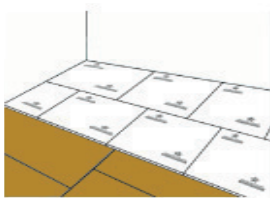
5. Check the subfloor is free from debris and completely flat. Minor differences in levels can be evened out by spreading a thin layer of tile adhesive on to the subfloor. Fix the 6mm Multi-Pro MoistSure board to the floor at 200mm fixing centres using countersunk screws.
