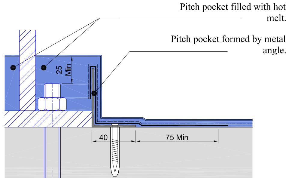
ENLARGED VIEW OF PITCH POCKET
