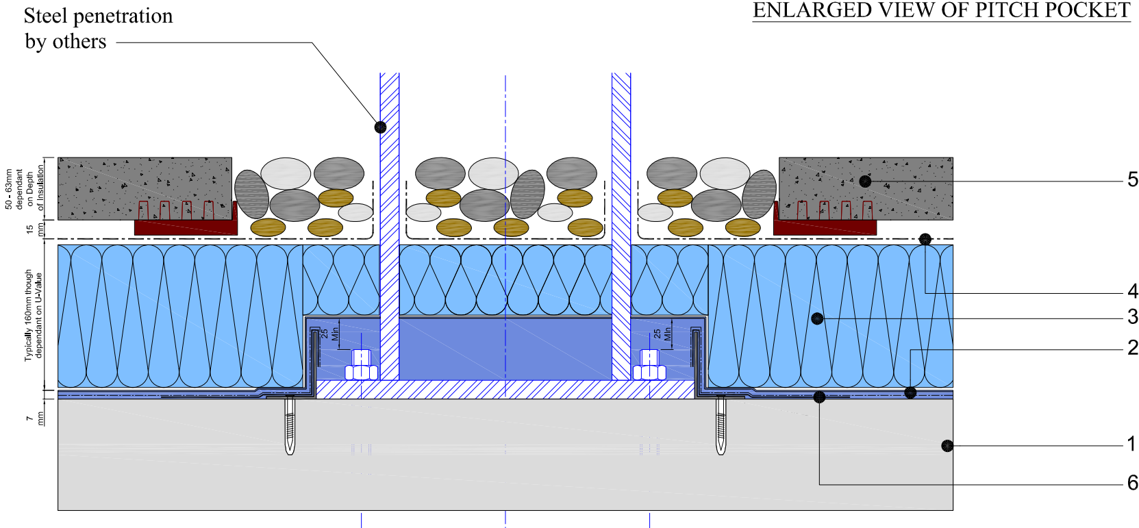
ENLARGED VIEW OF PITCH POCKET
