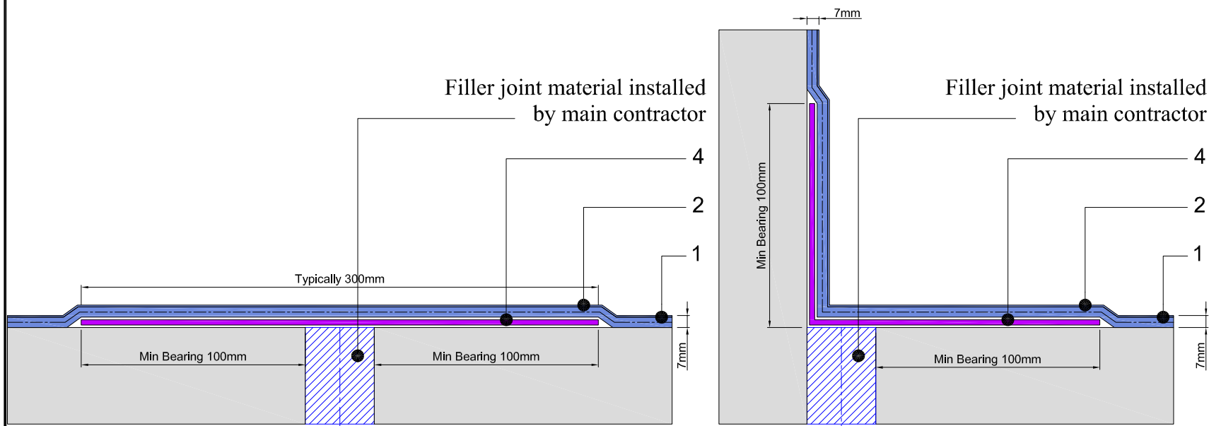
Waterproofing Expansion joints Greater than 12mm
