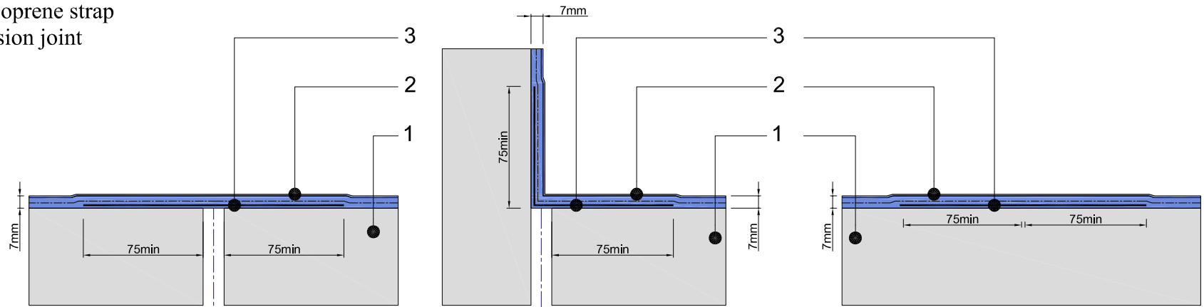
Waterproofing Expansion joints up to 12mm
