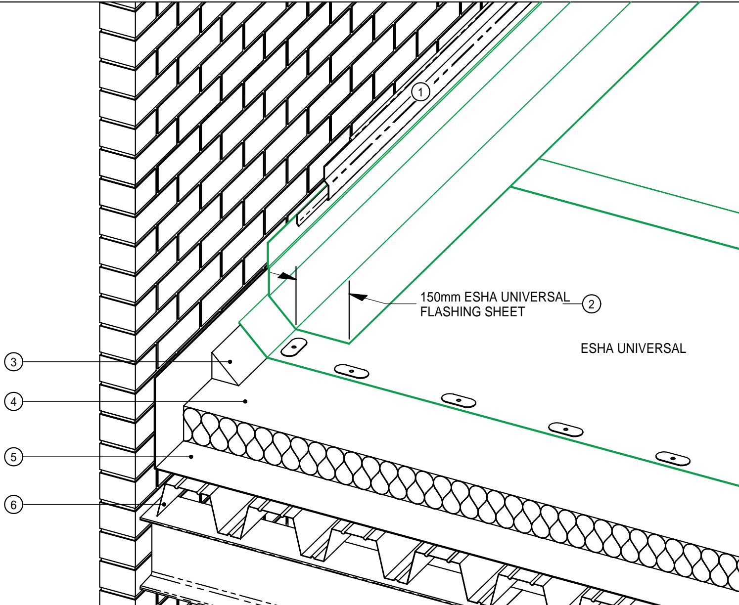
Section A - 9 Flashing to upstand, not insulated. New construction.
