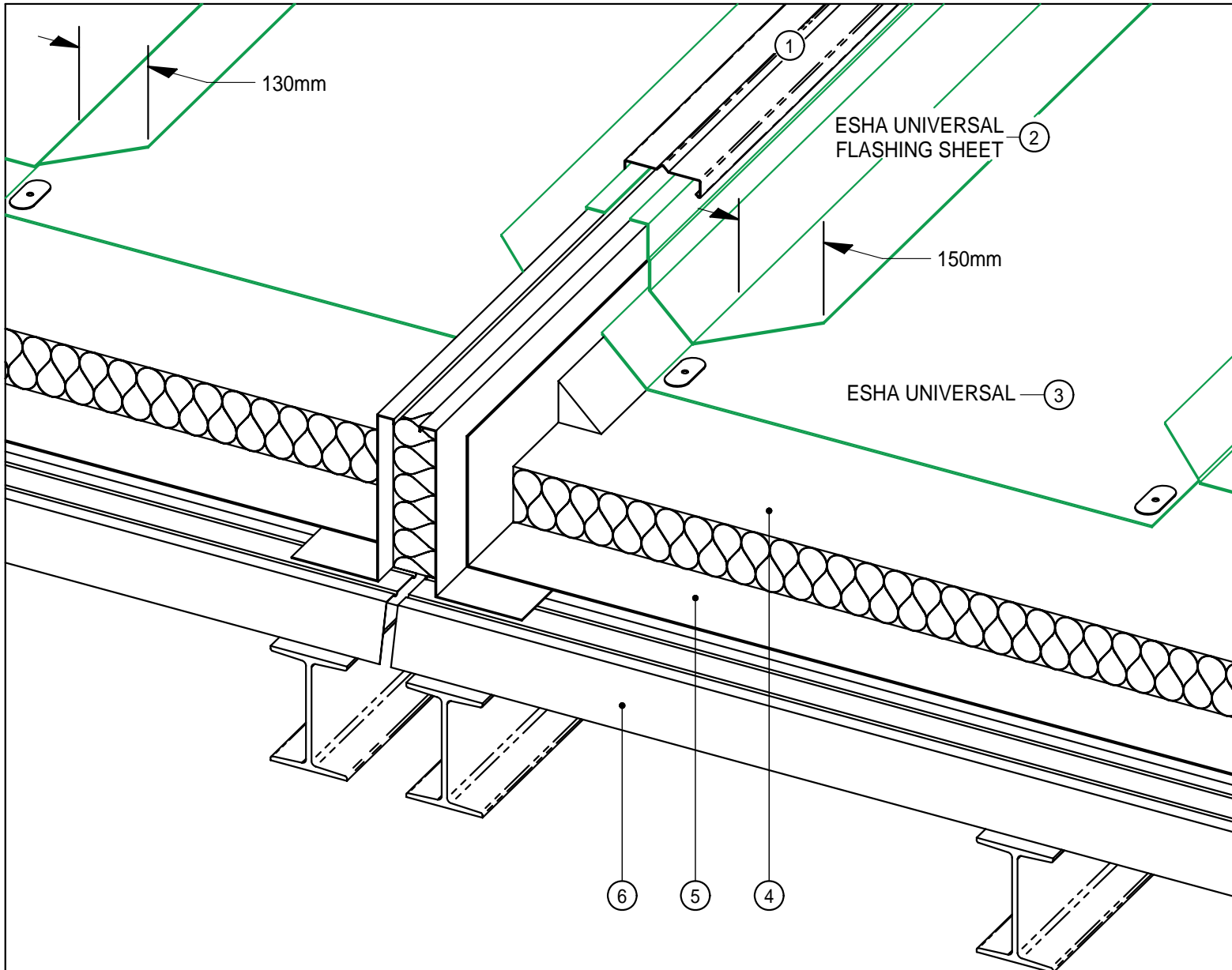
Section A - 11 Expansion ridge on roof surface. New Construction
