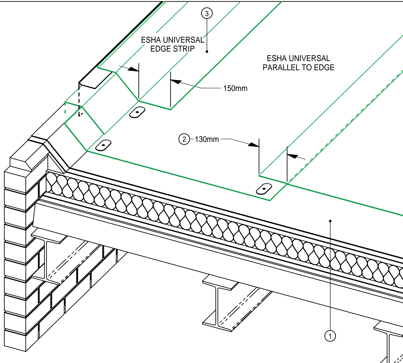
Section B - 6 Roof edge finish with roof edge profile. Refurbishment
