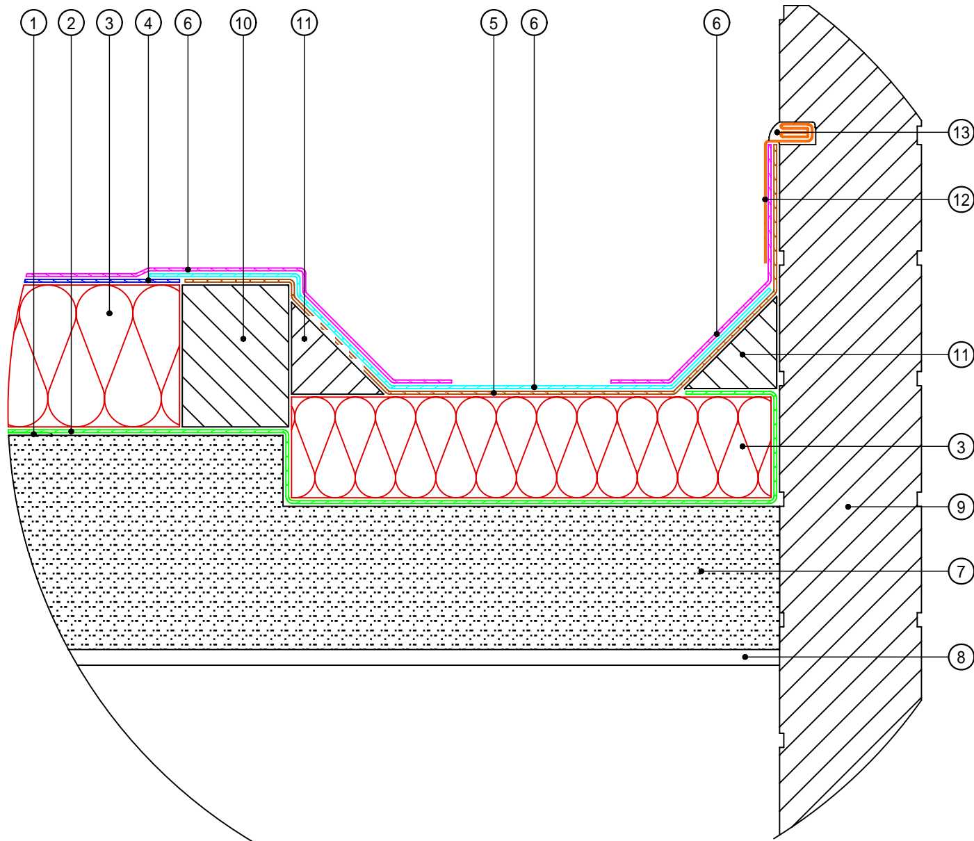
Section 11a Internal gutter detail
