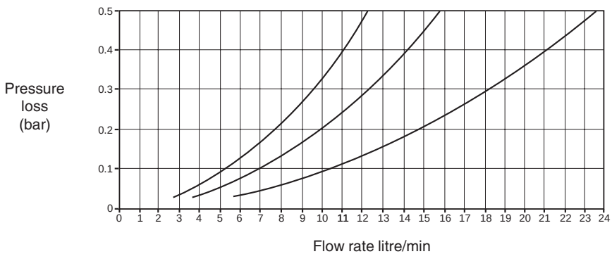
Shower fittings with high capacity spray plate
