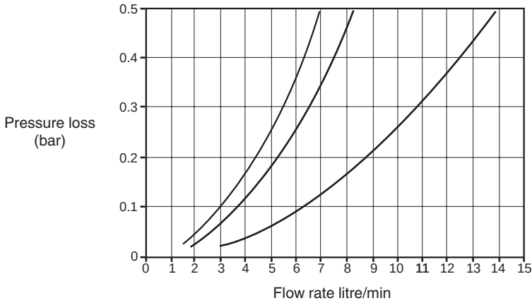
Shower fittings with low capacity spray plate
