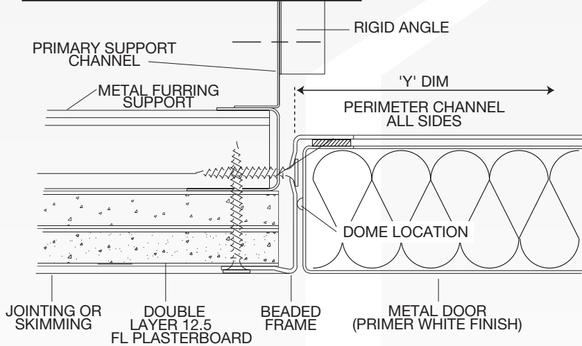
Fig.4 scale 1:2 section on B
