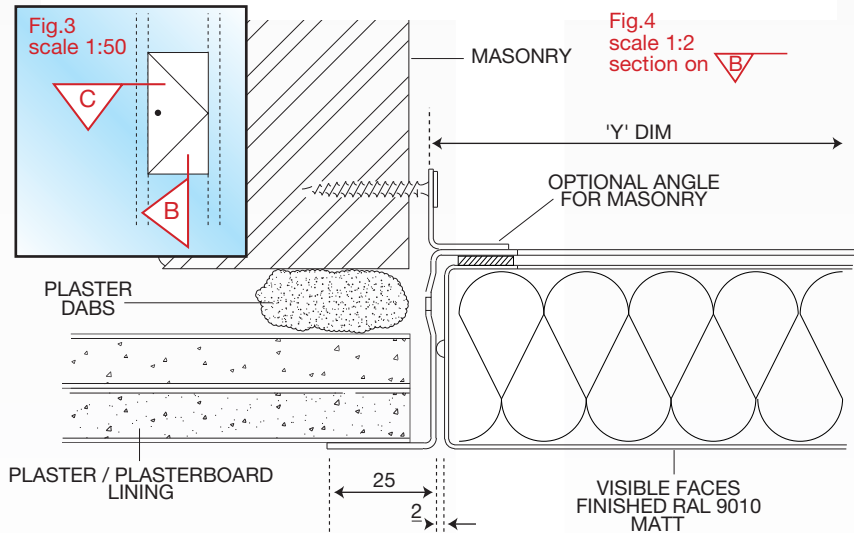
Fig.5 scale 1:2 section on C
