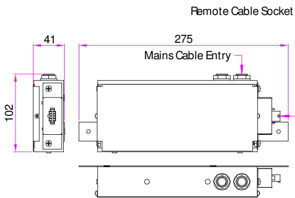
Remote Gear Box
