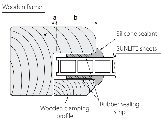
Figure 16b "Wet" Glazing
