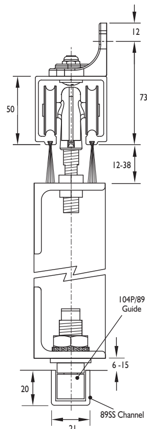
56/250/SS Hanger Face Fix
