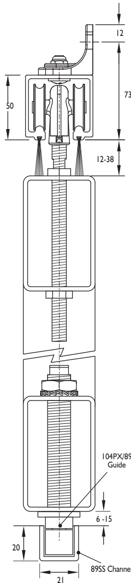
56X/250/SS Hanger Face Fix
